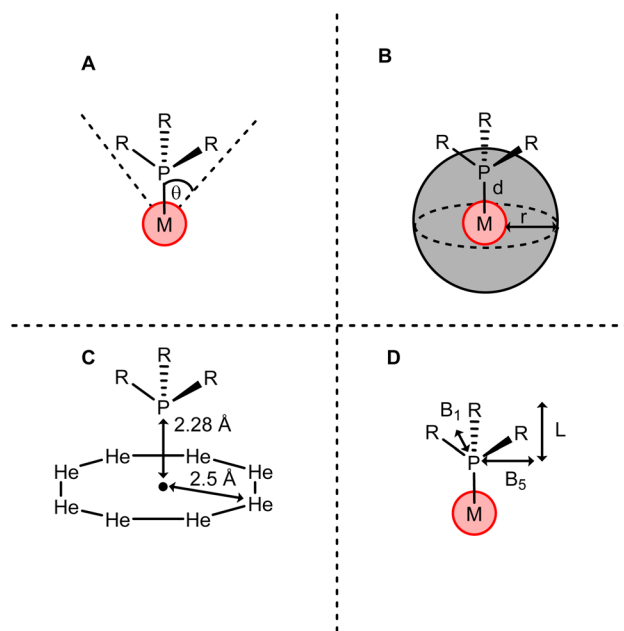
Fig. 16 Representation of steric calculation methods for a phosphine ligand \text{PR}_3 by (A) Tolman cone angle, (B) percentage buried volume, (C) \text{He}_s steric and (D) sterimol parameters.
