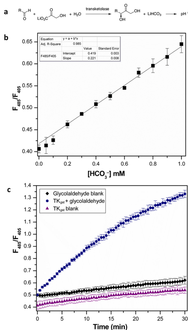
Fig. 2 (a) Transketolase reaction with pH shift. (b) Calibration curve of fluorescence intensity ratio ( \lambda_{\text{ex}} 485 \text{ nm}/\lambda_{\text{ex}} 405 \text{ nm} ) with NaHCO 3 standard (0–1 mM). All measurements were performed in triplicate. (c) Progress of transketolase reaction with 20 mM glycolaldehyde and 50 mM LiHPA. Error bars represent SD from triplicate measurements.
