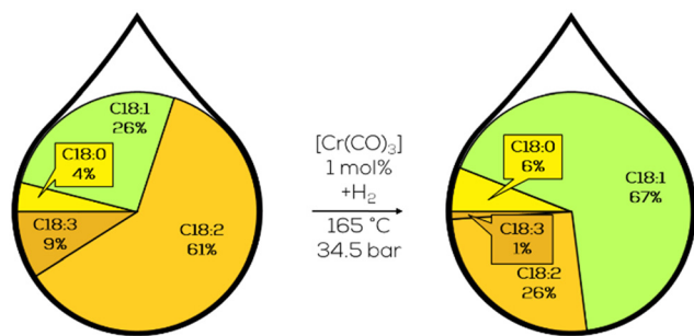
Fig. 31 C18 fatty acid composition in the hydrogenation of soybean oil by chromium carbonyl complexes as performed by Frankel et al. 172
