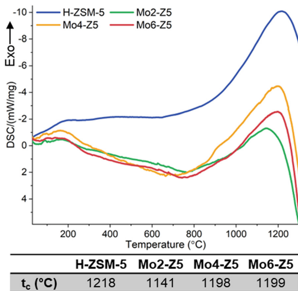
Fig. 4 DSC traces of H-ZSM-5, Mo2-Z5, Mo4-Z5, and Mo6-Z5. t_c s of the Mo exchanged H-ZSM-5 samples and H-form precursor are listed in Table 1. Note the weak shoulders at 900\text{ }^\circ\text{C} in the Mo4-Z5 and Mo6-Z5 samples are probably due to Mo volatilisation.
