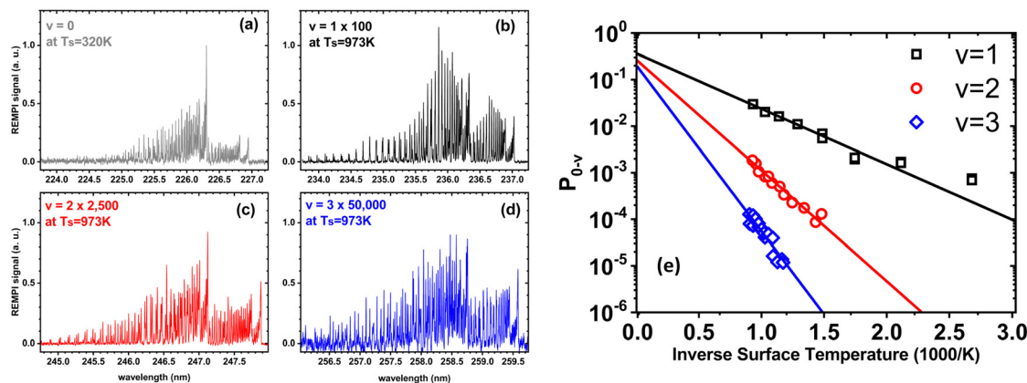
Fig. 1 Scattering of NO ( \nu = 0 ) from Au(111) at an incidence energy of translation of 0.4 eV. (a) REMPI spectrum of scattered NO ( \nu = 0 ) at a surface temperature of 320 K; (b)–(d) REMPI spectra of scattered NO ( \nu = 1, 2 and 3) when the surface temperature was 973 K. All REMPI spectra are normalized by transition strength, laser power and detection sensitivity. Note the different intensity multiplication factors, indicating different amounts of NO ( \nu = 0, 1, 2, 3 ) stemming from different population of thermally excited electron–hole pairs possessing sufficient energy to excite the corresponding vibrational state; (e) the temperature dependence of the excitation probabilities. Data-points – experiment, solid lines – fits to eqn (1) with A_{0,1} = 0.35 \pm 0.01 , A_{0,2} = 0.24 \pm 0.01 , and A_{0,3} = 0.16 \pm 0.01 . Data replotted from ref. 50.
