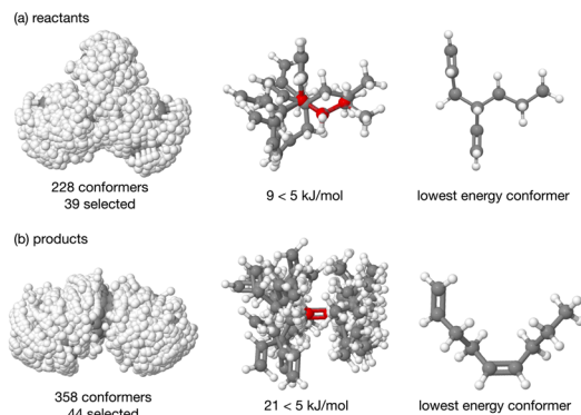
Fig. 2 Reaction A, overlay of all the CREST conformers (ball and stick) for the (a) reactants and (b) products, then only those evaluated to have energy <5 kJ mol -1 are depicted, the last image in each row is the lowest energy structure at the B3LYP level.
