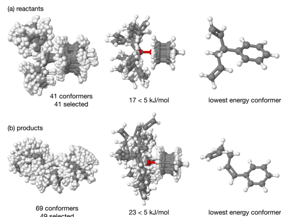
Fig. 3 Reaction B, Overlay of all the CREST conformers (ball and stick) for the (a) reactants and (b) products, then only those evaluated to have energy <5 kJ mol -1 are depicted, the last image in each row is the lowest energy structure at the B3LYP level.
