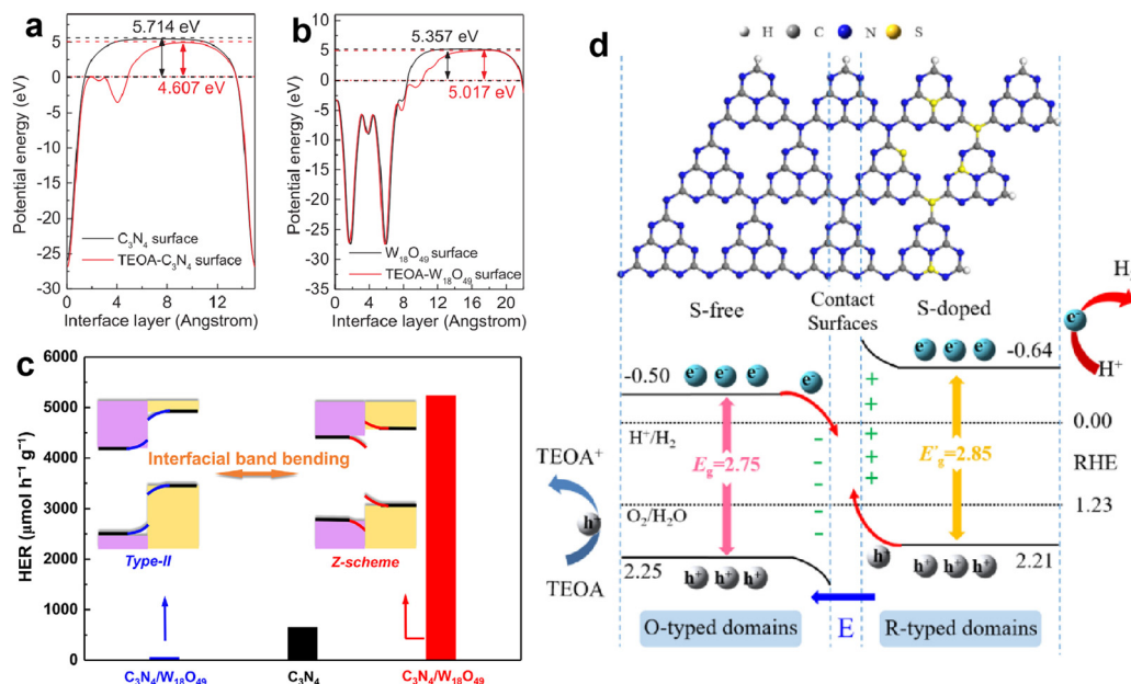
Fig. 9 The calculated work functions of g- C_3N_4 (a) and W_{18}O_{49} (b) surfaces with and without TEOA; photocatalytic H_2 evolution activities of pure g- C_3N_4 , type II g- C_3N_4 / W_{18}O_{49} , and Z-scheme g- C_3N_4 / W_{18}O_{49} (c). Reproduced with permission from ref. 116. Copyright 2017, Elsevier. The structural configuration and charge transfer mechanism of S-doped g- C_3N_4 /g- C_3N_4 isotype heterojunction (d). Reproduced with permission from ref. 131. Copyright 2022, Elsevier.
