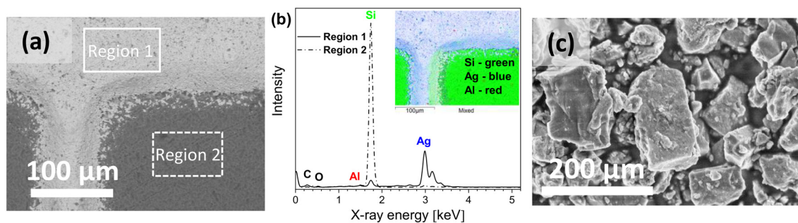
Fig. 1 SEM/EDS images showing: (a) EDS region analysis of the surface of the Si solar-cell sample, (b) EDS spectra for studied regions marked in image (a) (inset: EDS mapping image of the same sample showing distribution of Al, Si and Ag), and (c) SEM image of the ball-milled Si solar cells.
