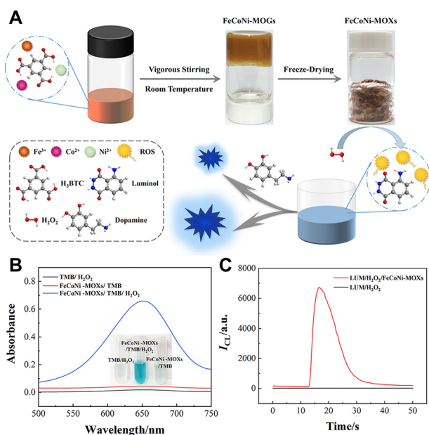
Fig. 10 (A) Schematic of the synthesis of \text{FeCoNi-MOXs} and its mechanism to enhance luminol/ \text{H}_2\text{O}_2 CL (B) UV-vis absorption spectra of the \text{TMB}/\text{H}_2\text{O}_2 , \text{FeCoNi-MOXs}/\text{TMB} , and \text{FeCoNi-MOXs}/\text{TMB}/\text{H}_2\text{O}_2 systems in 0.2 M \text{NaAc}/\text{HAc} buffer solution (ACB, pH 4.0). (C) CL intensity-time curves of the luminol/ \text{H}_2\text{O}_2 system in the absence and presence (red line) of \text{FeCoNi-MOXs} . [ \text{FeCoNi-MOXs} ]: 20 \mu\text{g mL}^{-1} ; [luminol]: 2 \mu\text{M} in CBS (pH 11.0); [ \text{H}_2\text{O}_2 ]: 20 \mu\text{M} . Reprinted with permission from ref. 62, Copyright 2023 American Chemical Society.
