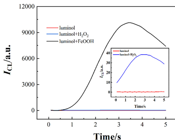
Fig. 11 The CL intensity-time curves of luminol, luminol/ \text{H}_2\text{O}_2 and luminol/ \text{FeOOH} systems. [Luminol]: 100 \mu\text{M} ; [ \text{FeOOH} ]: 25 \mu\text{g mL}^{-1} ; [ \text{H}_2\text{O}_2 ]: 1 \mu\text{M} ; [pH]: 10.0. Reprinted with permission from ref. 63, Copyright 2023, American Chemical Society.
