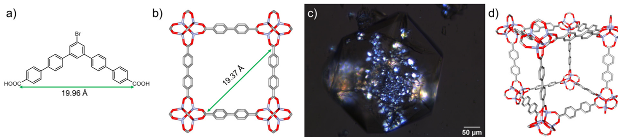
Fig. 1 (a) Molecular structure of designed additive: 5''-bromo-[1,1':4',1'':3'',1''':4''',1''':4''']-quinquephenyl]-4,4''''-dicarboxylic acid. (b) Structure of pore window in the {100} plane of IRMOF-10. C–C distances are highlighted in green. (c) Image of IRMOF-9/10 crystal synthesized with additive under polarized light illustrating a mixture of birefringent (noncubic) and crystallographically cubic regions. (d) Structure of a single cage of IRMOF-10 obtained via single crystal X-ray diffraction. Non-disordered structure depicted and hydrogen atoms omitted for clarity.
