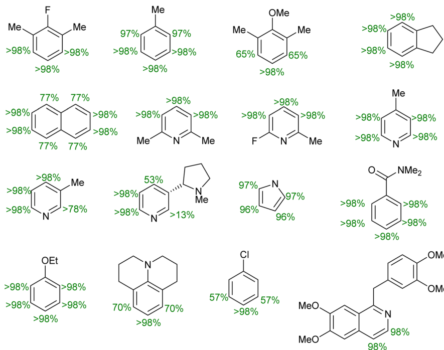
Scheme 14 Substrate scope for HIE reaction using 36 .
