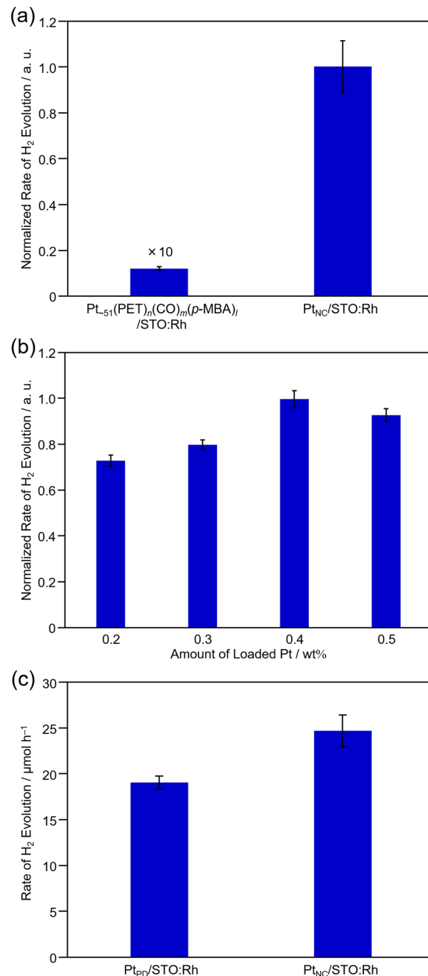
Fig. 5 H 2 -evolution activity of Pt cocatalyst-loaded STO:Rh photocatalysts. (a) Before ( \text{Pt}_{51}(\text{PET})_6(\text{CO})_6(\text{p-MBA})_6/\text{STO:Rh} ) and after ( \text{Pt}_{\text{NC}}/\text{STO:Rh} ) calcination of Pt NC-loaded STO:Rh and (b) dependence of loading weight of the Pt cocatalyst for \text{Pt}_{\text{NC}}/\text{STO:Rh} . (c) Comparison of H 2 -evolution activity between \text{Pt}_{\text{NC}}/\text{STO:Rh} and \text{Pt}_{\text{PD}}/\text{STO:Rh} . In (a) and (c), the loading weight of Pt on them was 0.4 wt%. In order to eliminate the effect of the difference in the activity of each photocatalyst, STO:Rh synthesized in the same batch was used in each experiment (a)–(c).
