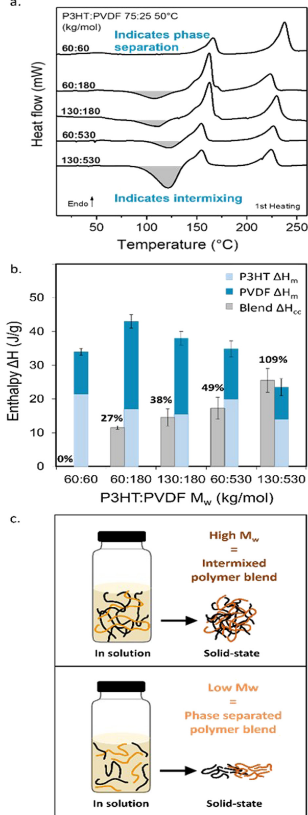
Fig. 2 Using molecular weight as a tool to manipulate the extent of vitrification in solution-processed blends. (a) DSC first heating thermograms measured on solution-processed blends of P3HT and PVDF of different molecular weights. More pronounced cold-crystallization exotherms (CC, shaded in grey) are observed for blends comprising higher molecular weight components. (b) Comparison of \Delta H_{cc} and the combined
