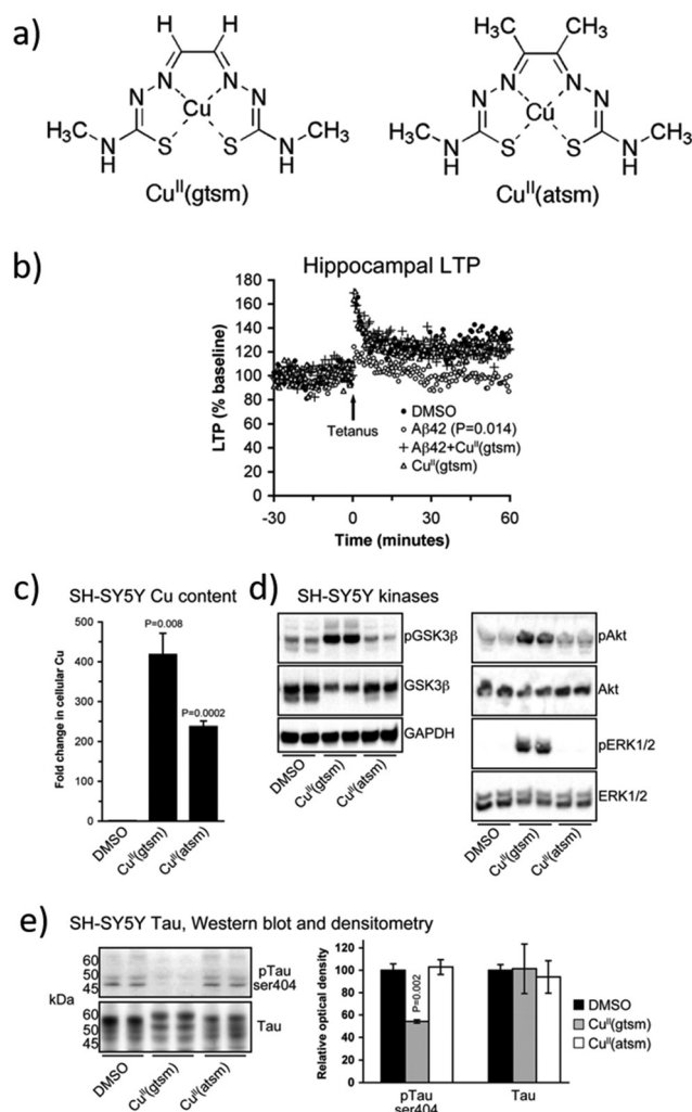
Fig. 5 (a) Structures of [Cu II (gtsm)] and the control [Cu II (atsm)]. (b) Whereas Aβ 42 inhibits the hippocampal long-term potentiation (LTP) by 28%, this is prevented when treated with [Cu II (gtsm)]. (c) In vitro , [Cu II (gtsm)] increases the cellular levels of Cu. (d) Western blot analyses show that [Cu II (gtsm)] induces the phosphorylation of kinases GSK3β, Akt, and ERK1/2. (e) [Cu II (gtsm)] inhibits tau phosphorylation at ser404 without affecting the abundance of total tau. Adapted from Ref. 68. Reproduced with permission.
