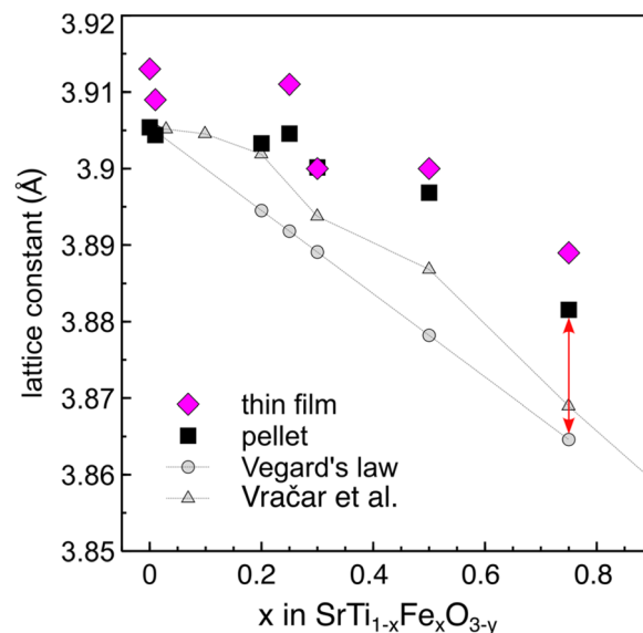
Fig. 5 X-Ray diffraction. Refined lattice constants from the XRD patterns of \text{Sr}(\text{Ti},\text{Fe})\text{O}_{3-y} thin films and pellets as a function of the iron content. For comparison, we show Vegard's law prediction based on oxidized \text{Sr}(\text{Ti},\text{Fe})\text{O}_3 solid solutions and the results of powders oxidized under 600 bar \text{O}_2 from Vračar et al. 43,46,69
