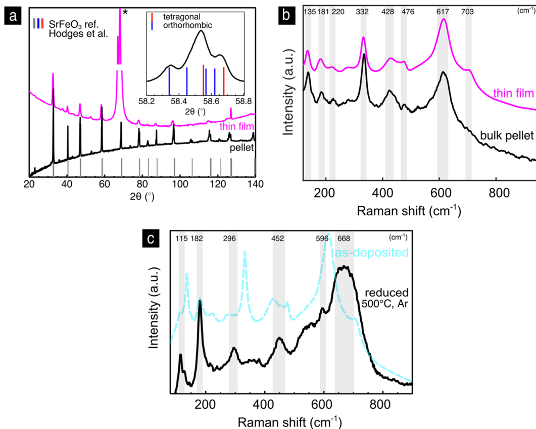
Fig. 4 Strontium iron oxide, \text{SrFeO}_{3-y} : (a) XRD-pattern of the thin film and bulk pellet with an inset of a sample reflection from the bulk pellet with a reference of the tetragonal and orthorhombic phases. (b) Raman spectra of the \text{SrFeO}_{3-y} thin film and bulk pellet. (c) Comparison of the Raman spectra of the as-deposited and reduced thin films.
