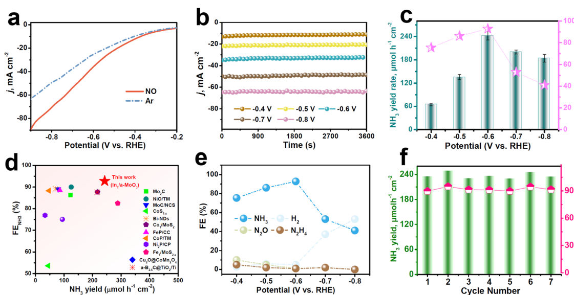
Fig. 3 (a) LSV curves of \text{In}_1/\text{a-MoO}_3 in Ar/NO-saturated 0.5 M \text{Na}_2\text{SO}_4 at a rate of 10 \text{ mV s}^{-1} . (b) Chronoamperometry test of \text{In}_1/\text{a-MoO}_3 at various potentials, and resulting (c) \text{NH}_3 yield rates and \text{FE}_{\text{NH}_3} . (d) Comparison of \text{NH}_3 yields and \text{FE}_{\text{NH}_3} between \text{In}_1/\text{a-MoO}_3 and reported NORR catalysts. (e) FEs of different products on \text{In}_1/\text{a-MoO}_3 after NORR electrolysis at various potentials. (f) Cycling test of \text{In}_1/\text{a-MoO}_3 at -0.6 \text{ V} .
