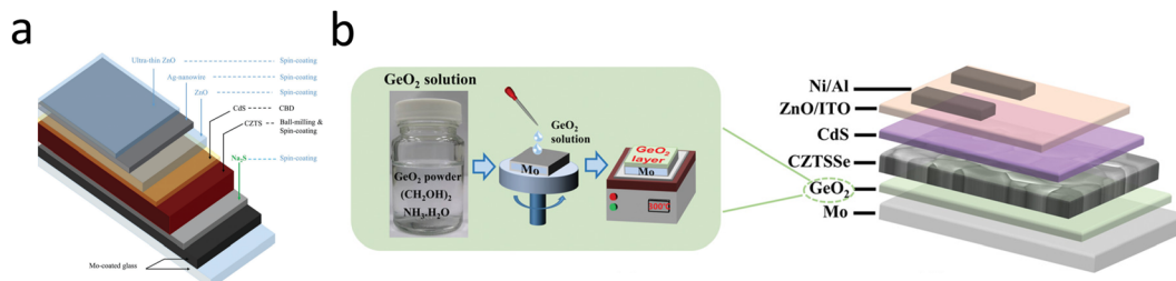
Fig. 4 (a) Schematic diagram of CZTS solar cells. 43 Reproduced with permission from ref. 43. (b) Schematic diagram of CZTSSe devices containing \text{GeO}_2 layers. 46 Reproduced with permission from ref. 46.
