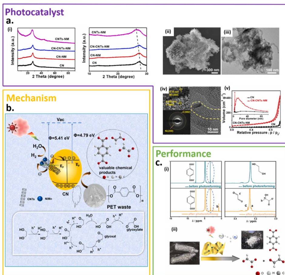
Fig. 8 (a) (i) XRD patterns of CN, CN-NiMo, CN-CNTs-NiMo and CNTs-NiMo. (ii) SEM images of CN-CNTs-NiMo. (iii) Low-magnification TEM and (iv) HRTEM image and SAED pattern of CN-CNTs-NiMo. (v) N 2 adsorption-desorption isotherms of CN-CNTs-NiMo and CN. (b) Schematic diagram of the process of photoreforming of PET using CN-CNTs-NiMo. (c) (i) 1 H NMR spectra of PET before and after photoreforming. (ii) Photoreforming of PET to obtain commodity chemicals and H 2 fuel. Reaction conditions: 10 mL KOH (5 M), pretreated PET (50 mg mL -1 ), and 10 mg CN-CNTs-NiMo under simulated solar light for 4 h at 288 K. Light resource: simulated solar light, 95 mW cm -2 . Reproduced with permission from ref. 93. Copyright 2022, Elsevier.
