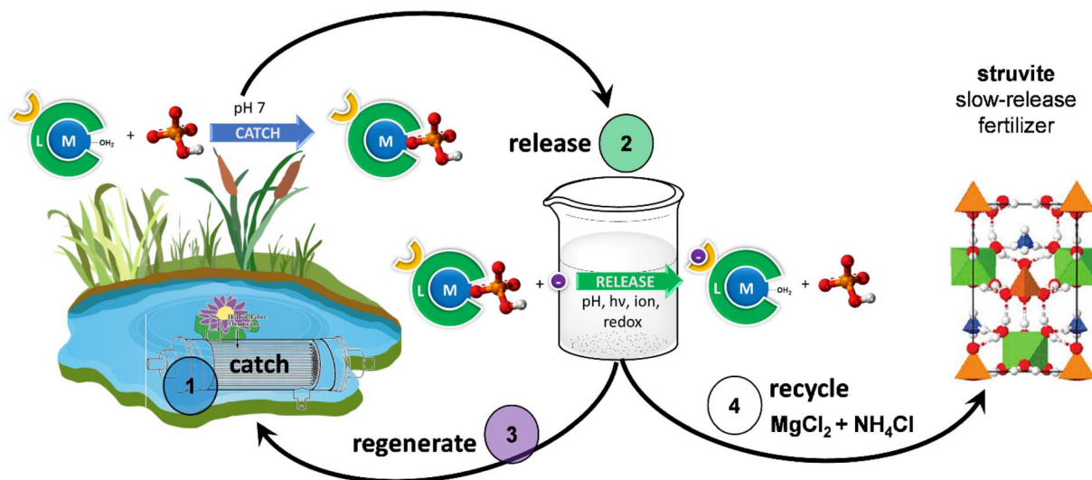
Fig. 2 A proposed cycle of catch-and-release with regenerable lanthanide receptors to remediate polluting phosphate into struvite fertilizer. Affinity for phosphate is controlled via reversible instillation of peripheral negative charge on the receptor. Image reproduced courtesy of Dr. Valérie Pierre.
