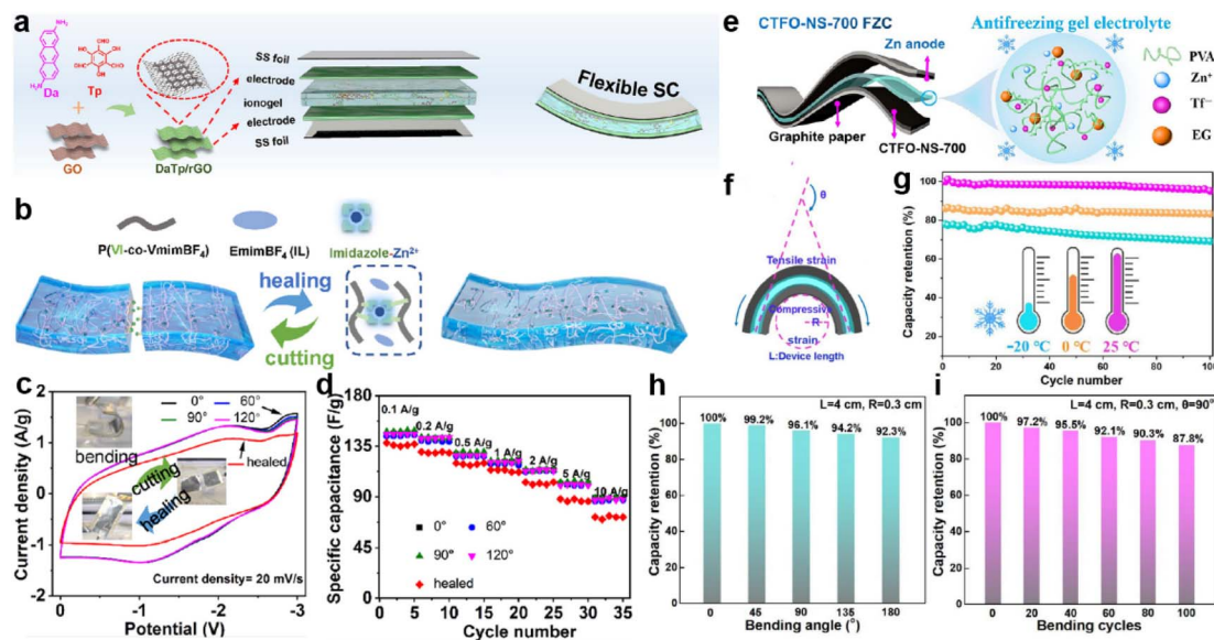
Fig. 16 (a) Schematic of FSCs assembled from P_{28}/Zn^{2+}/2IL ion gel-electrolyte and DaTp/rGO electrodes. (b) Schematic of the spontaneous self-healing ionogel using Im-Zn^{2+} interaction as a dynamic motif. (c) CV curves of FSC with different bending angles and healed FSC. (d) Rate performance of FSCs with different bending angles and the healed sample. Reprinted from ref. 132. Copyright 2023, Elsevier. (e) Schematic structure of CTFO-NS-700 FZC and freeze-resistant PVA/ Zn(Tf)_2 /EG gel electrolyte. (f) Schematic diagrams of the structure and bending state of CTFO-NS-700FZC, (h) capacity retention at different bending angles, and (i) capacity retention after 100 bending cycles. (g) Capacity retention of CTFO-NS-700 FZC at 25 °C, 0 °C, and 20 °C. Reprinted from ref. 138. Copyright 2023, Elsevier.
