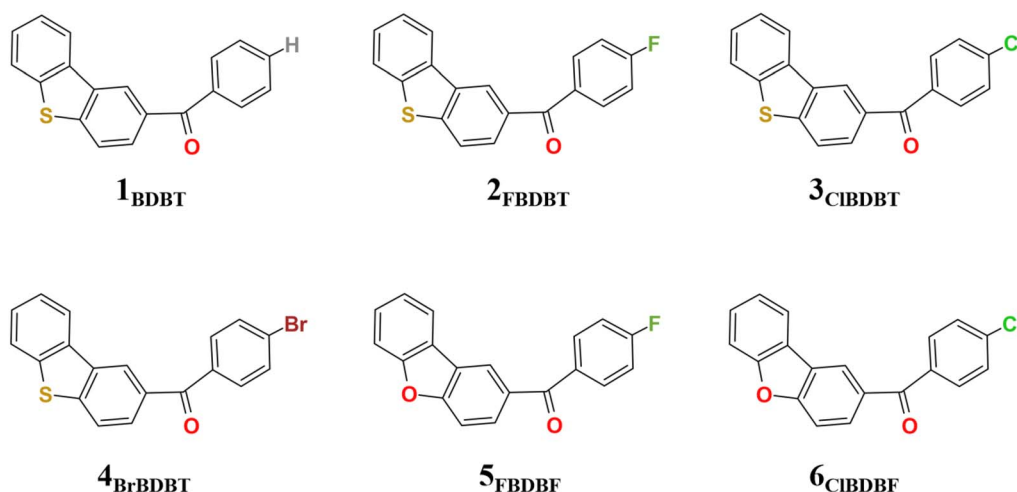
Fig. 1 Geometrical structures for 1 BDBT , 2 FBDBT , 3 ClBDT , 4 BrBDBT , 5 FBDBF , and 6 ClBDFF .
