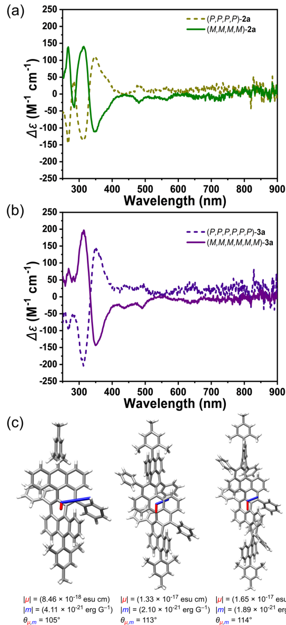
Fig. 4 (a and b) CD spectra of (P,P,P,P)- 2a , (M,M,M,M)- 2a , (P,P,P,P,P,P)- 3a , (M,M,M,M,M,M)- 3a measured in dichloromethane at 25 °C with different concentrations ( c = 1.34 \times 10^{-5} M, 1.84 \times 10^{-5} M, 6.93 \times 10^{-6} M, 1.87 \times 10^{-5} M, respectively). (c) Calculated transition dipole moments for S_0 \rightarrow S_1 electronic transitions in (P,P)- 1a , (P,P,P,P)- 2a , (P,P,P,P,P,P)- 3a . The electric transition moments ( \mu ) are shown in red, and the magnetic transition moments ( m ) are shown in blue. The length of the \mu vector is minified by 100 times when the length of the m vector is amplified by 100 times for clarity.
