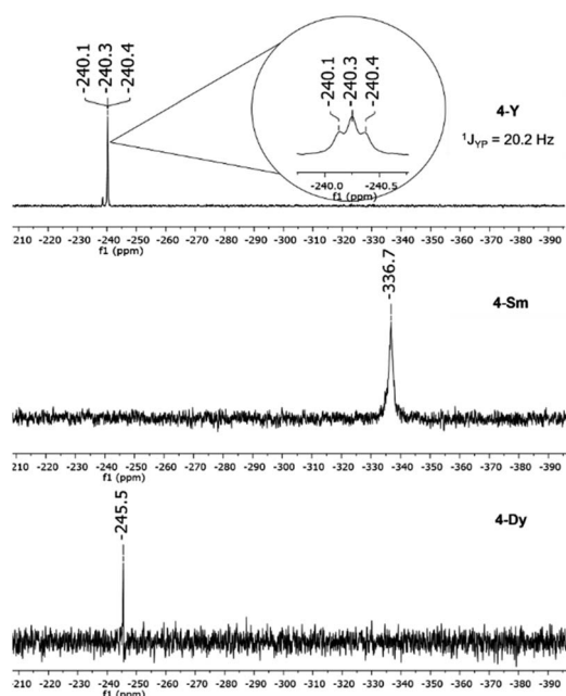
Fig. 6 ^{31}\text{P}\{^1\text{H}\} NMR spectra of [\text{K}(\text{NON})\text{Ln}^{\text{III}}(\text{thf})_2(\mu_3\text{-}\eta^3\text{:}\eta^2\text{-P}_3)] ( 4-Ln ) in \text{thf-d}_8 at 25^\circ\text{C} .
