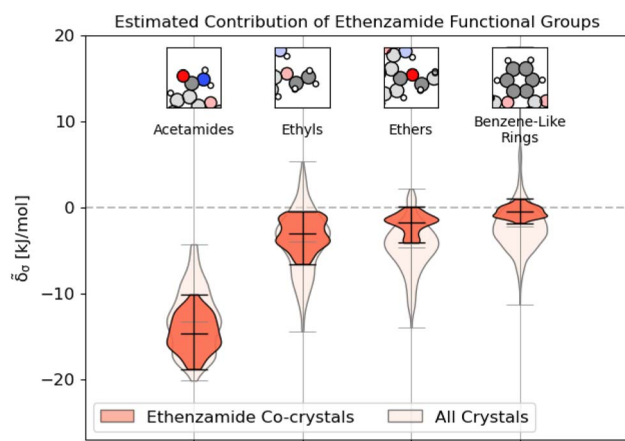
Fig. 9 Distribution of energetic contributions for the functional groups of ethenzamide. Following the procedure outlined in 3.2, we have computed the estimated contribution to the binding energy \hat{\delta}_o . Similar to Fig. 2, we have arranged the functional groups in order of average contribution, and the lines on each plot denote each group's extreme and mean contributions. Wider sections of the violin plot represent a higher probability that members of the population will take on the given value; the skinnier sections represent a lower probability. Here, darker sections refer to the distribution in the functional groups of the ethenzamide molecules, with lighter sections showing the distribution for the same functional group across the entire training set.
