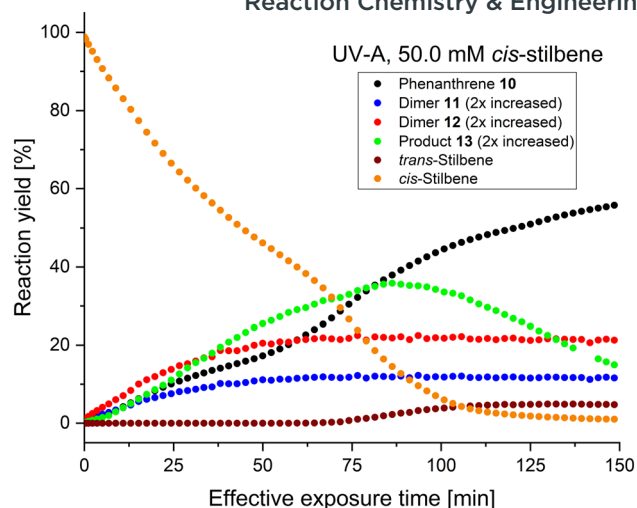
Fig. 7 GC results from the switch-off experiments of Mallory photoreaction using 50.0 mM cis -stilbene and UV-A light source.
