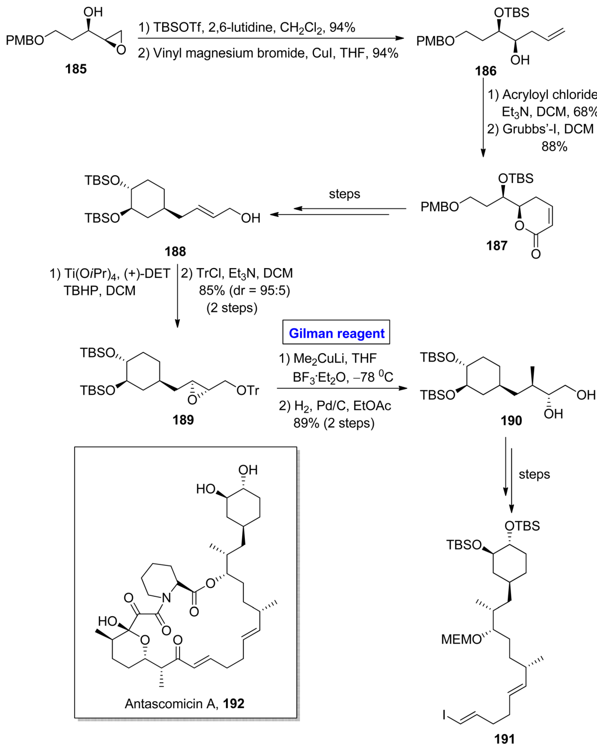
Scheme 21 Synthesis of the C17–C34 fragment 191 towards the synthesis of antascomicin A 192 .
