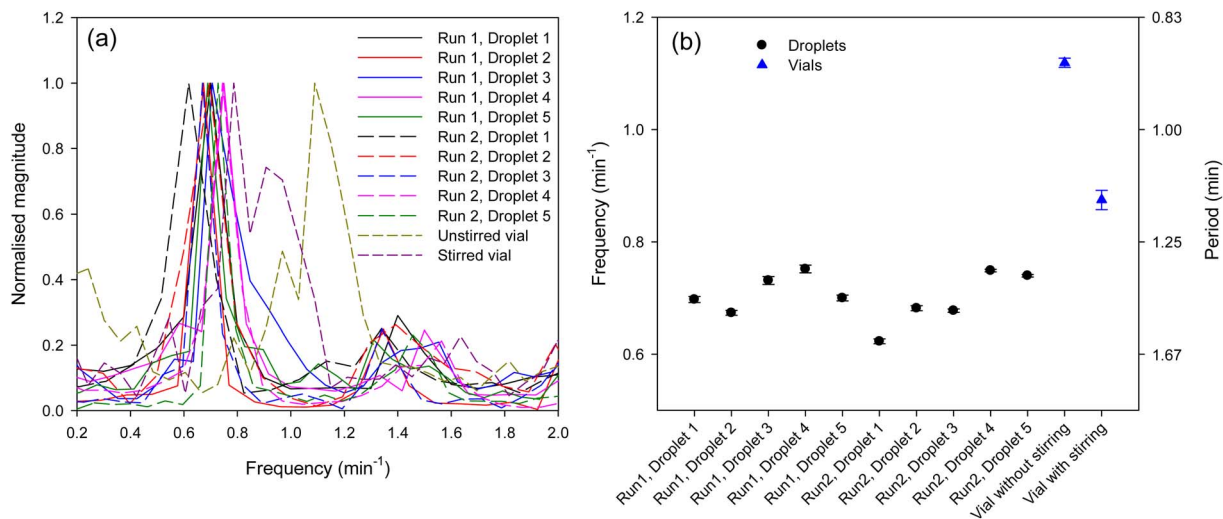
Fig. 6 (a) FFTs of the entire time courses for two runs with five droplets of 1 \times mixture levitated simultaneously and in the unstirred and stirred vials and (b) scatter plot with error bars ( \pm 1 standard deviation) of the oscillation period derived from the FFTs.
