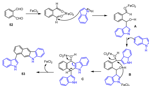
Scheme 37 Proposed mechanism for Fe-catalyzed cycloaddition reaction.
