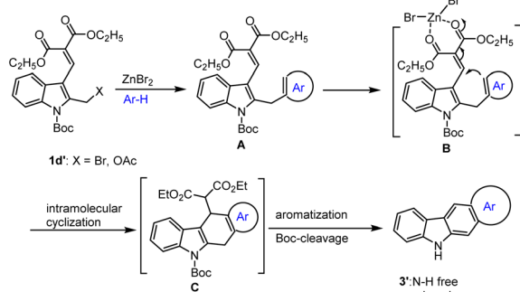
Scheme 9 Proposed mechanism for domino reaction of N -Boc-bromomethyl indole enabled by \text{ZnBr}_2 .
