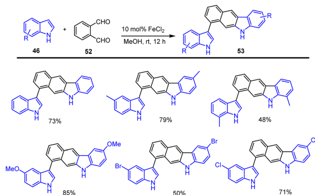
Scheme 36 Fe-catalyzed cycloaddition of indoles and o -phthalaldehyde.
