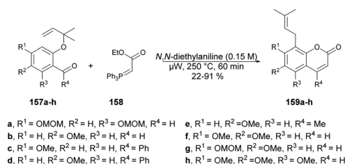
Scheme 56 Synthesis of 8-prenylcoumarins 159a-h .
