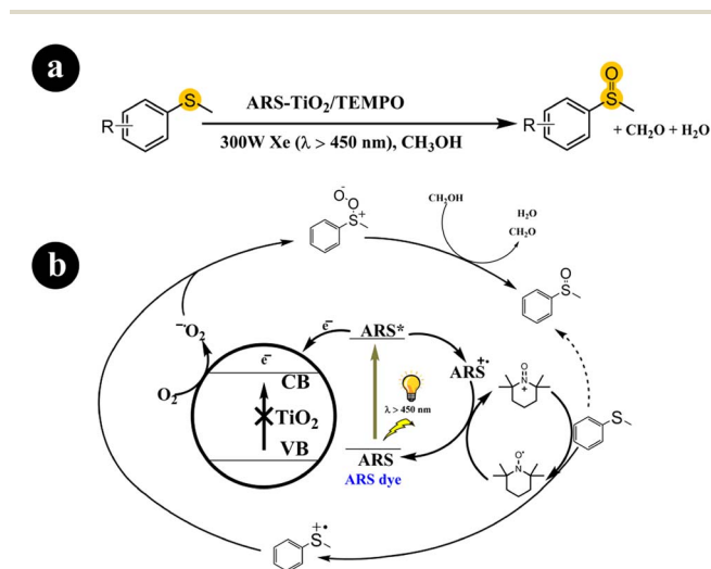
Scheme 5 (a) The reaction conditions for this process include specific parameters such as the type of catalyst (ARS-sensitized TiO 2 ), the presence of a co-catalyst (TEMPO), the use of visible light as the energy source, and the involvement of molecular oxygen (aerobic conditions). (b) One potential mechanistic route for the visible light photocatalytic aerobic oxidation of thioanisole involves ARS-sensitized TiO 2 and TEMPO. Reproduced with permission from ref. 40. Copyright 2016, John Wiley and Sons.
