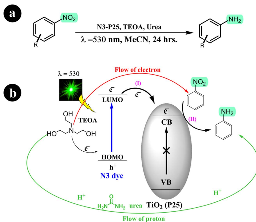
Scheme 15 (a) The conversion reaction and the conditions for the catalysis system; (b) the reduction of nitrobenzene through photocatalysis using dye-sensitized \text{TiO}_2 is achieved in the presence of urea, which acts as a mediator for proton transfer. Reproduced from ref. 56 with permission, copyright 2011, Royal Society of Chemistry.
