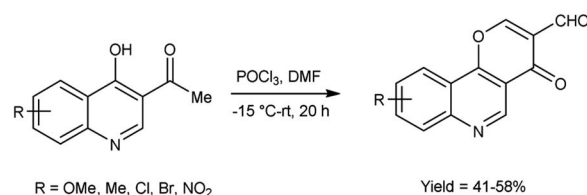
Scheme 48 Synthesis of pyrano[3,2- c ]quinolone-3-carbaldehydes.
