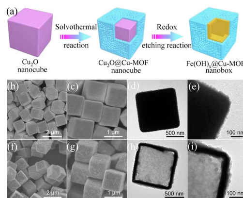
Fig. 7 Synthesis and characterization of \text{Fe}(\text{OH})_x@ -Cu-MOF NBs. (a) Schematic illustration of the synthetic process for \text{Fe}(\text{OH})_x@ -Cu-MOF NBs. (b and c) FESEM images of \text{Cu}_2\text{O}@ -Cu-MOF NBs. (d and e) TEM images of \text{Cu}_2\text{O}@ -Cu-MOF NBs. (f and g) FESEM images of \text{Fe}(\text{OH})_x@ -Cu-MOF NBs. (h and i) TEM images of \text{Fe}(\text{OH})_x@ -Cu-MOF NBs. Reproduced from ref. 90 with permission from Amer Assoc Advancement Science, Copyright 2021.
