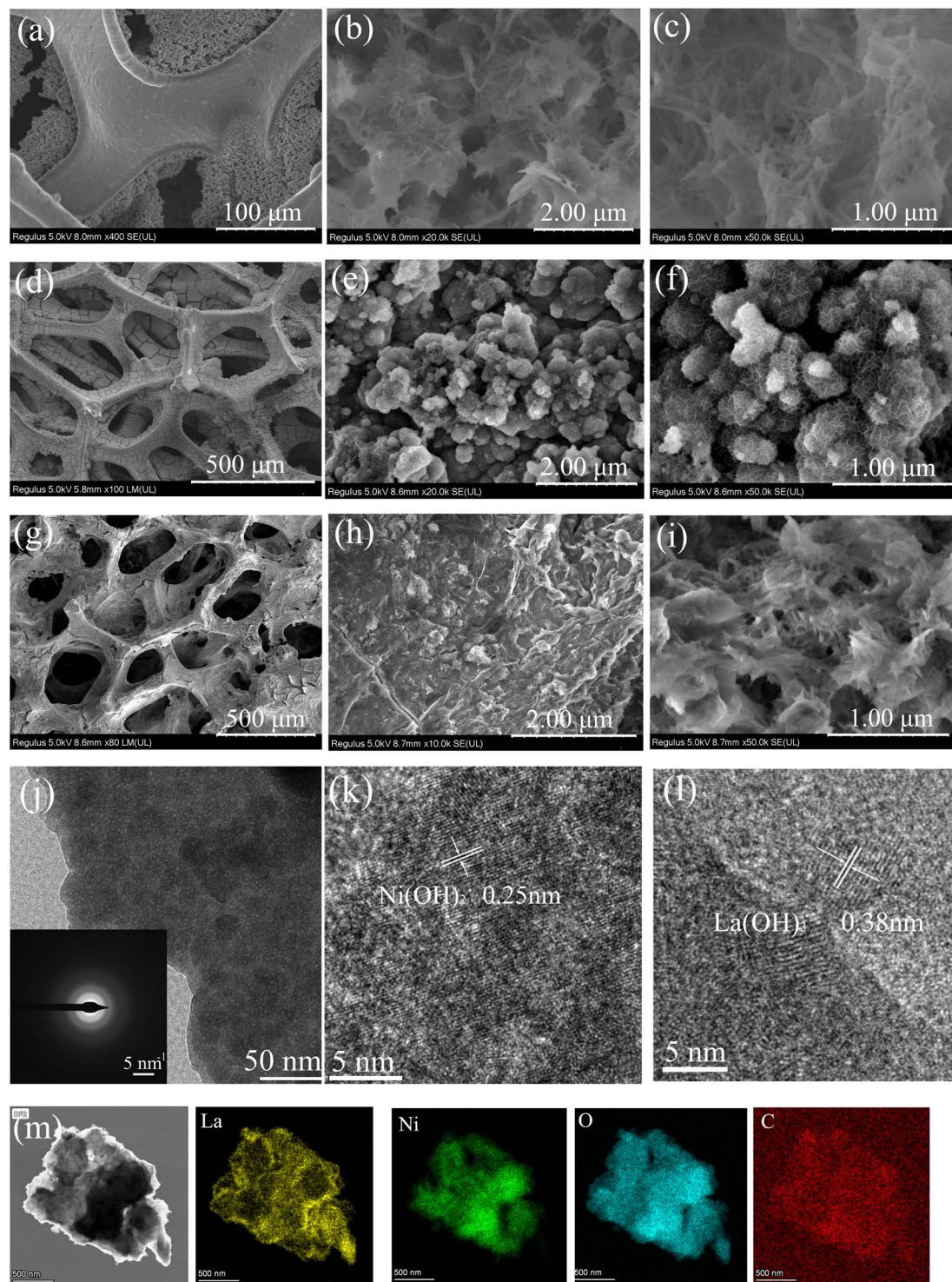
Fig. 1 SEM images of \text{La}(\text{OH})_3/\text{CG} (a)–(c), \text{Ni}(\text{OH})_2/\text{CG} (d)–(f) and \text{La}@\text{Ni}/\text{CG} (g)–(i); TEM images of \text{La}@\text{Ni}/\text{CG} (j) and insert SAED pattern; HRTEM images of \text{La}@\text{Ni}/\text{CG} (k) and (l); TEM images of \text{La}@\text{Ni}/\text{CG} and corresponding mappings of La, Ni, O and C (m).
