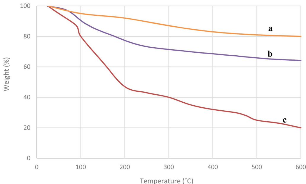
Fig. 7 TGA analysis of (a) \text{Fe}_3\text{O}_4 , (b) \text{SiO}_2@\text{Fe}_3\text{O}_4 , and (c) \text{Ni}^{\text{II}} -picolylamine/TCT/APTES@ \text{SiO}_2@\text{Fe}_3\text{O}_4 .
