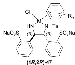
M = Ru(II), \eta^6 -arene: e = p -Cymene, f = benzene, g = mesitylene, h = 4- tert -ButylToluene \eta^6 -arene = Cp*, M: i = Rh(II), j = Ir(II)
