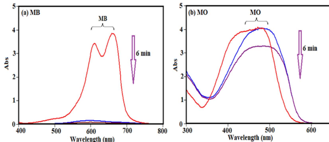
Fig. 12 The UV-vis spectra during adsorption of (a) cationic MB and (b) anionic MO dyes over the \text{H}_3\text{PW}_{12}\text{O}_{40}/\text{Fe}_3\text{O}_4/\text{MIL-88A (Fe)} : C_o (dye) = 30 \text{ mg L}^{-1} , V_{\text{dye}} = 30 \text{ mL} , adsorbent dosage = 20 \text{ mg} , temp = 25^\circ\text{C} .
