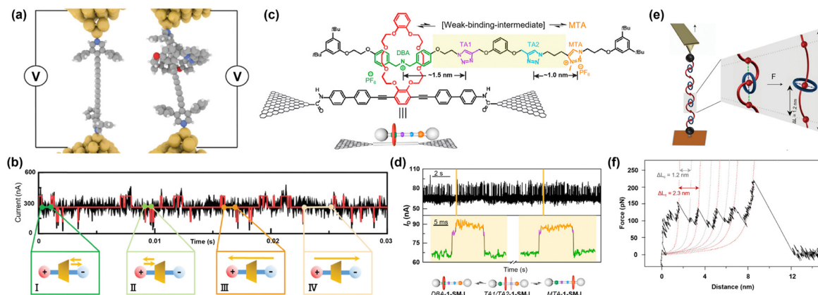
Fig. 8 (a) Schematic representation of conductance measurement in the STM single-molecule junction. (left) Oligoyne guest molecule (right) after rotaxation. Reprinted with permission of ref. 171. Copyright 2017 Royal Society of Chemistry. (b) Current–time measurement based on which the signal is categorized into four possible shuttling scenarios. (I) Two consecutive high-conductance states (II), two consecutive low-conductance states (III), complete shuttling from the high-conductance state to the middle-conductance and then to the low-conductance state and (IV) from the low-conductance state to the middle-conductance and then to the high-conductance state. Reprinted with permission of ref. 172. Copyright 2019 Wiley. (c) Structure of the molecular shuttle threaded inside a crown ether. The axle features MTA and DBA units and two intermediate TA1 and TA2 binding sites. (d) (top) Real-time current measurement conducted for 1-SMJ inside the DMSO environment at 338 K. (bottom) Expanded region of the current–time curve indicated by yellow lines. The intermediate conductance states corresponding to TA1/TA2 binding sites are labeled purple. These short-lived co-conformers occur during transitions of the macrocycle between DBA (green) and MTA (orange). Reprinted with permission of ref. 173. Copyright 2022 Elsevier. (e) Schematic of the cantilever retraction process at a constant velocity. The mechanical elongation leads to the breaking of the non-covalent interaction between a DNP and adjacent ring, and consequently, mechanical unfolding. (f) Force–distance curve recorded at a low speed of 40 \text{ nm s}^{-1} demonstrating a sawtooth profile with existing second peaks. Reprinted with permission of ref. 176. Copyright 2018 Springer Nature.
