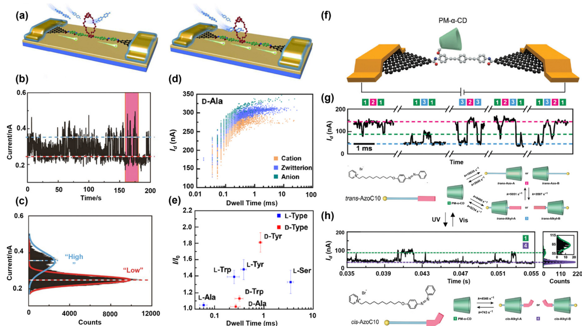
Fig. 6 (a) Schematic representations of the graphene–molecular–graphene junction consisting of (left) BPP34C10, which has a lower conductance, and (right) a more conductive host–guest system when a charged molecule of MV2+ passes through the host's cavity. (b) Measured current as a function of time for BPP34C10-SMJ once it is immersed in a solution containing MV2+, and (c) the corresponding 1D histogram for the current measurement showing bimodal conductance states. Reprinted with permission of ref. 136. Copyright 2016 Science. (d) Current versus dwell time 2D histogram for L-Ala at pH = 7. (e) Conductance variation ( I/I_0 ) as a function of dwell time used as enantiomer recognition for various amino acids. I_0 is the basic current for empty PM- \beta -CD. Reprinted with permission of ref. 111. Copyright 2021 Science. (f) Schematic of the GMGJ nanodevice consisting of a photosensitive single supramolecular junction. Current–time signal and molecular structure in (g) trans and (h) cis form under visible light and UV, respectively, showing a reversible binding process. Reprinted with permission of ref. 110. Copyright 2022 Wiley.
