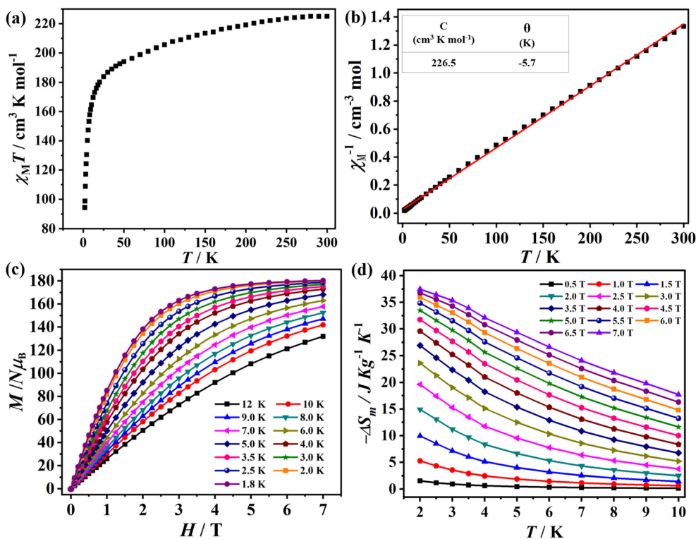
Fig. 6 (a) Plot of experimental magnetic susceptibility ( \chi_M T ) versus T ; (b) \chi_M^{-1} versus T plot; (c) plot of M – H under different T temperatures; and (d) plot of experimental magnetic entropy change ( -\Delta S_m ) versus T for Gd 28 .
