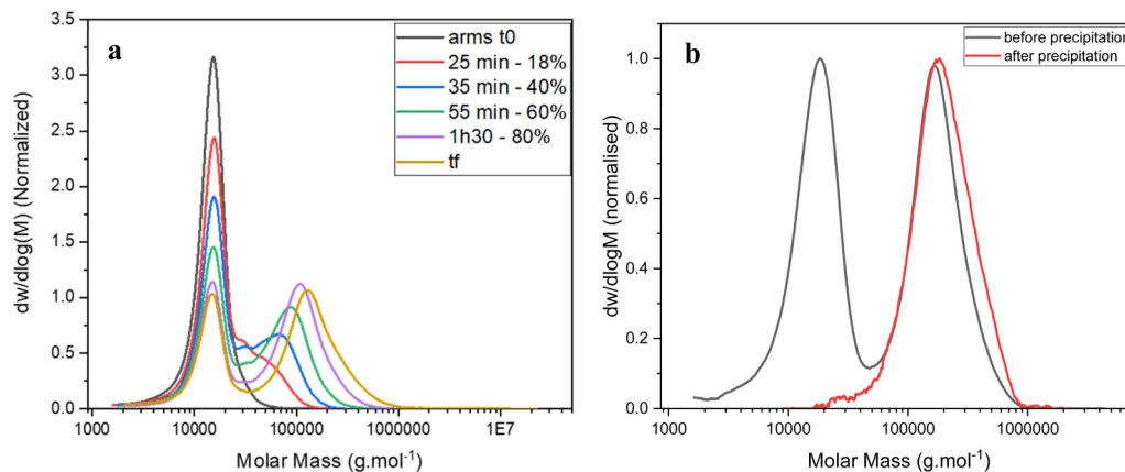
Fig. 2 GPC traces of (a) the kinetic of star formation ( [CL] = 0.2 M, [CL]/[mCTA] = 3 , [mCTA]/[I] = 20 ) – samples are taken at 0 minute ( t_0 ), 25, 35 and 90 minutes and at the end of the reaction ( t_f – 180 minutes; 95% crosslinker conversion) – the percentage corresponds to the crosslinker conversion measured by ^1\text{H} NMR; (b) star polymer at t_f and after purification by precipitation, showing complete removal of unreacted arms.
