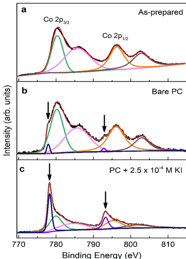
Fig. 5 X-ray photoelectron spectra of Co 2p 3/2 and Co 2p 1/2 for (a) as-prepared, (b) treated in bare PC and (c) PC + 2.5 \times 10^{-4} M KI samples. The downward arrows point to the Co 2p 3/2 and Co 2p 1/2 peaks of metallic Co (in blue and purple in (b) and (c)). Additionally, green and orange correspond to Co 2+ , and pink and brown to Co 3+ . Solid black lines are experimental data, whereas solid red lines refer to fitting spectra.
