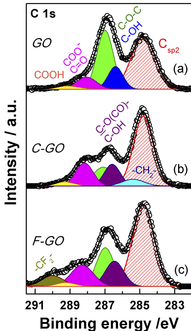
Fig. 7 XPS spectra in the region C 1s of GO (a), C-GO (b), and F-GO (c). Experimental data are reported in dots, while fitting reconstruction is represented by a continuous line and color-filled curves corresponding to the various functional groups. Color code: red: \text{sp}^2 C=C; blue: hydroxyl; green: epoxy; magenta: carbonyl/carboxylate; yellow: carboxyl; light cyan: methylene; violet: ester/hydroxyl (see text); dark yellow: di-fluoromethylene.
