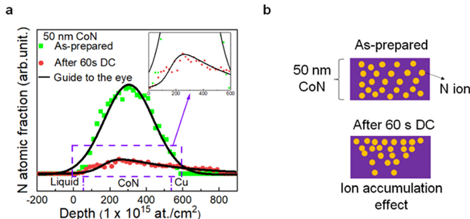
Fig. 4 Direct proof of the ion accumulation effect. (a) Elastic recoil detection measurements revealing the N depth distribution of an as-prepared and an actuated (–25 V DC voltage for 60 s) 50 nm-thick film, with a zoomed-in view of the area surrounded by the purple dashed box. (b) Cartoon representing the N ion distribution in an as-prepared sample and an actuated sample showing the ion accumulation effect.
