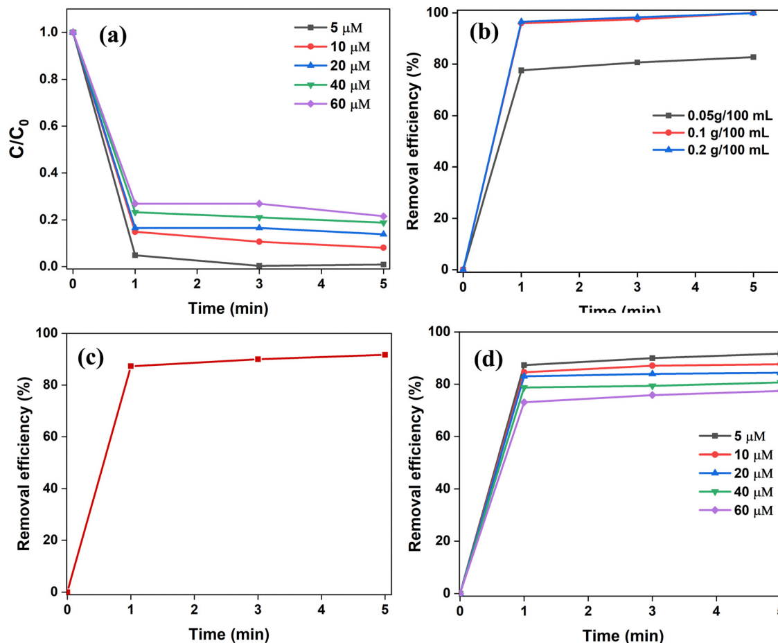
Fig. 6 (a) Adsorption efficiencies of spherical SnO 2 NPs as observed for various dye concentrations; (b) effect of adsorbent dosage on the removal efficiency for 5 μM CR at pH = 5; (c) effect of contact time upon the removal efficiency for 5 μM CR dye; and (d) effect of dye concentration on the removal efficiency for CR by 0.1 g/100 mL of SnO 2 NPs.
