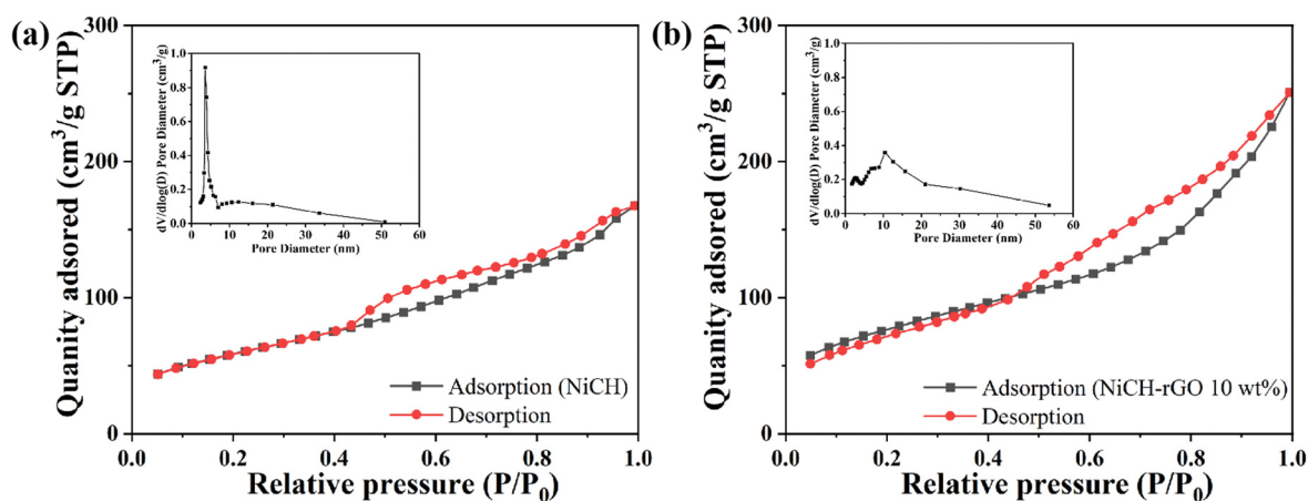
Fig. 5 \text{N}_2 adsorption–desorption isotherms of (a) NiCH and (b) NiCH–rGO 10 wt%. Insets are the corresponding pore size distribution curves of the corresponding sample.
