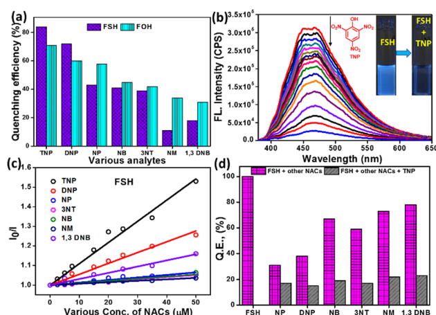
Fig. 3 (a) Variation in the quenching efficiency of 1 \mu\text{M} of FOH and FSH treated with various nitrated analytes (500 \mu\text{M} ) in THF. (b) Changes in the emission intensity of FSH (1 \mu\text{M} ) upon treatment with various concentrations of TNP (500 \mu\text{M} ) in THF. (c) Stern–Volmer plot of FSH (1 \mu\text{M} ) was treated with 50 \mu\text{M} of various nitro analytes. (d) Interference study of FSH (1 \mu\text{M} ) with TNP (500 \mu\text{M} ) in the presence of other analytes (500 \mu\text{M} ).
