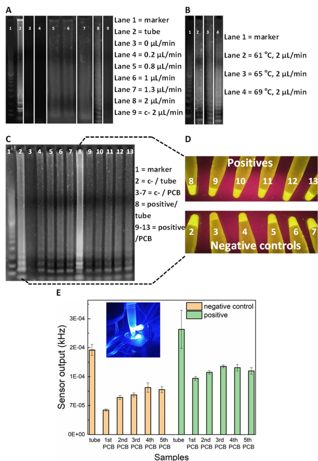
Fig. 2 Agarose gel electrophoresis after performing LAMP on PCB A) at 65 °C using various flow rates (lane 2 shows product derived from the tube heated using dry-block incubator) and B) using 2 μL min -1 at various temperatures. DNA marker 100 bp is shown in Lane 1. Synthetic SARS-CoV-2 DNA was used as template ( 2 \times 10^4 gc μL -1 ). C) Lanes 2 and 8 show negative control and positive heated in tube (using dry-block incubator) and lanes 3–7 and 9–13 show negative controls and positives derived from the PCB, respectively. Two PCB channels were used for lanes 3–7 and 9–13, one for the negative controls and one for the positives, to evaluate the reusability of the PCB channel. Synthetic SARS-CoV-2 DNA was used as template ( 2 \times 10^4 gc μL -1 ). D) Photographic images of tubes under UV light which contain the remaining samples after the gel loading of Fig. 2C and E) optical sensor output for the same samples that are shown in Fig. 2D (bars represent standard deviations of three measurements for each tube).
