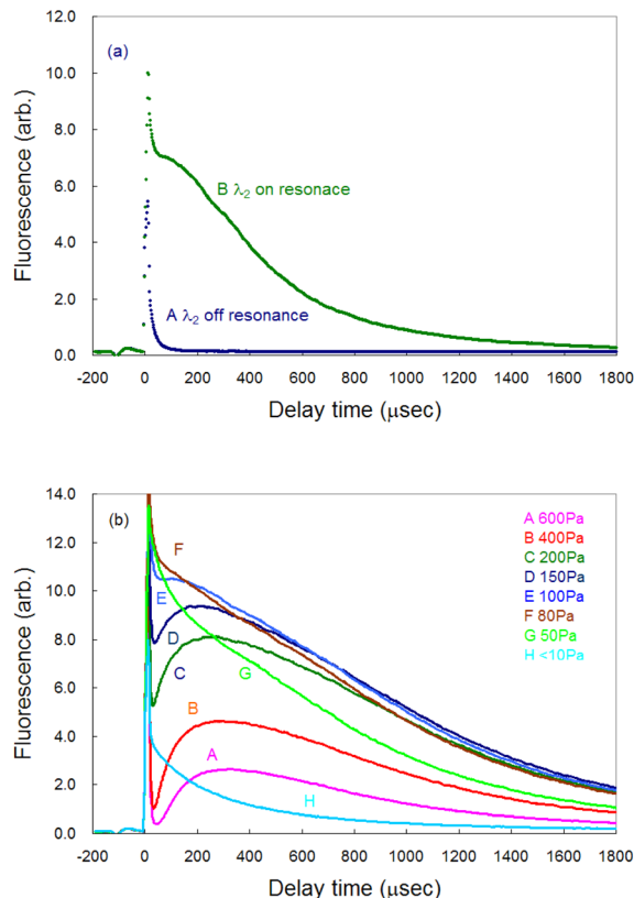
Fig. 3 (a) Temporal variation in the measured fluorescence signal of Ca and (b) its pressure dependence. Immediately after ablation, plasma emission was transmitted through the interference filter and overlapped with the fluorescence signal. The fluorescence signal had the highest intensity under about 100 Pa of helium.
