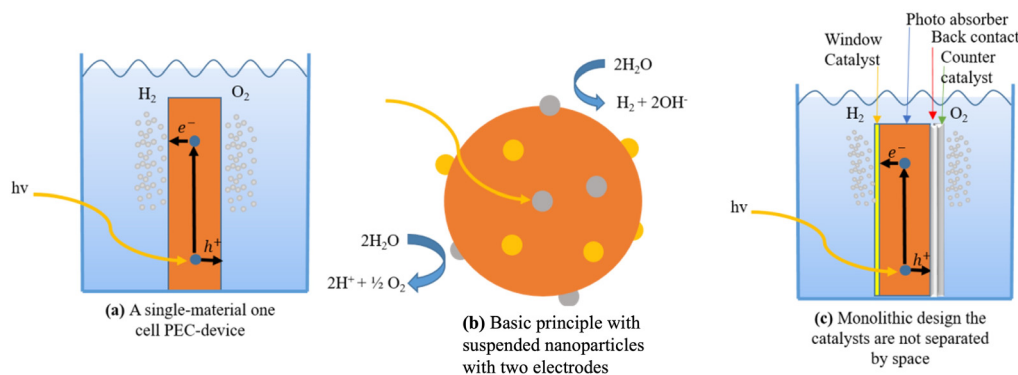
Fig. 16 (a) A single-material one-cell PEC-device. (b) Basic principle with suspended nanoparticles with two electrodes. (c) Monolithic design where the catalysts are not separated by space.
