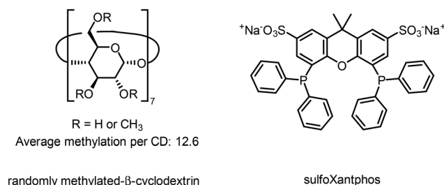
Fig. 4 Chemical structures of randomly methylated- \beta -cyclodextrin (phase transfer agent) and sulfoXantphos (ligand).
