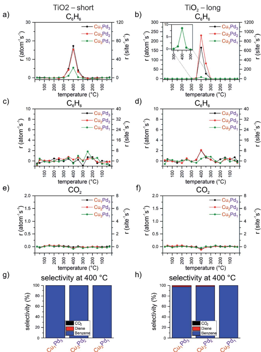
Fig. 3 Performance of \text{Cu}_1\text{Pd}_3 , \text{Cu}_2\text{Pd}_2 and \text{Cu}_3\text{Pd}_1 clusters on \text{TiO}_2 . Carbon-based per total atom and per site rates of \text{Cu}_m\text{Pd}_n on \text{TiO}_2 for the "short" and "long" ramps: (a) benzene – short, (b) benzene – long, (c) cyclohexadiene – short, (d) cyclohexadiene – long, (e) \text{CO}_2 – short, (f) \text{CO}_2 – long; carbon-based selectivity for benzene, cyclohexadiene and \text{CO}_2 at 400 ^{\circ}\text{C} during (g) the short ramp and (h) the long ramp ("short" refers to the first temperature ramp of the applied double ramp, with a dwell time of 20 minutes at 400 ^{\circ}\text{C} ; "long" refers to the second temperature ramp with a 2 hour dwell time at 400 ^{\circ}\text{C} ).
